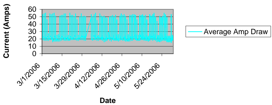
Average Amp Draw Across 3 Phases - 208V - 3/06 - 5/06
