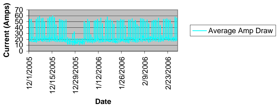
Average Amp Draw Across 3 Phases - 208V - 12/05-2/06
