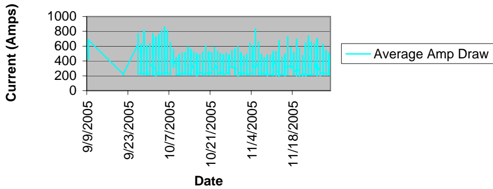
Average Amp Draw Across 3 Phases - 480V - 9/05-11/05
