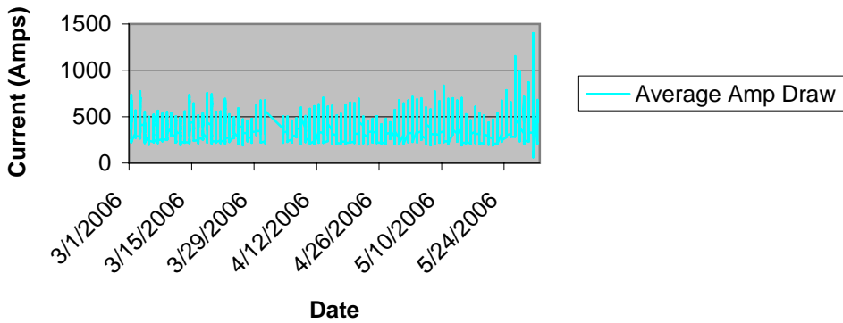
Average Amp Draw Across 3 Phases - 480V - 3/06-5/06
